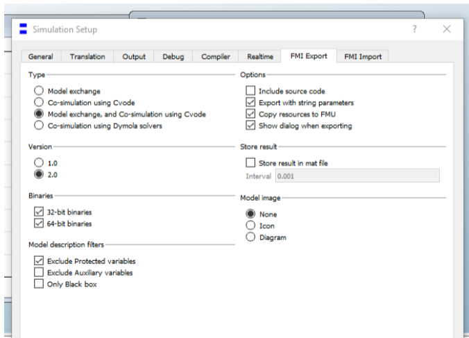
FMI export options in Dymola. Source: Claytex.
