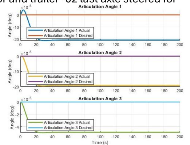
Steering Angle
