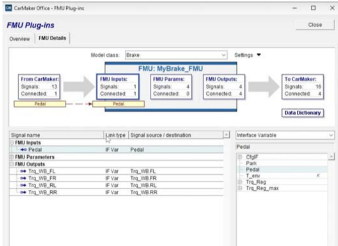
FMU details in CarMaker. Source: IPG Automotive.
