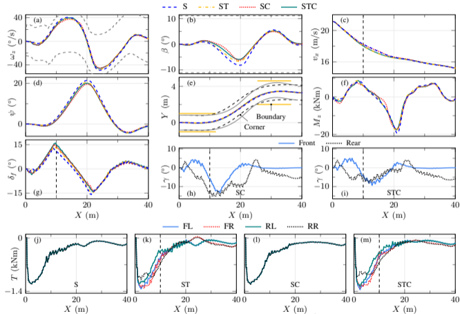
Trajectory tracking results 4 .
