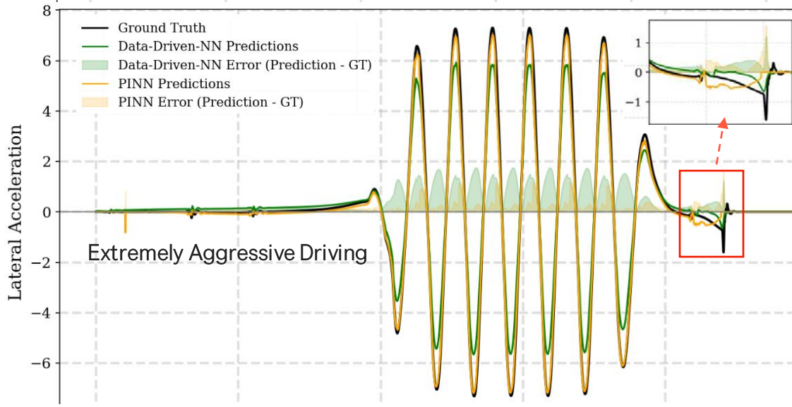
Prediction and Error on Lateral Acceleration(m/s 2 )
