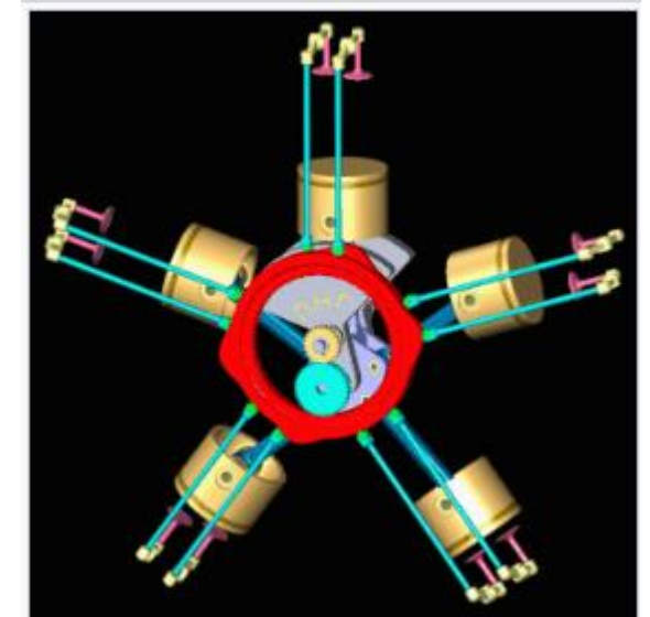
Source: Radial engine, Wikipedia
