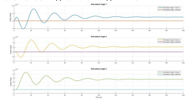
Articulation Angle
