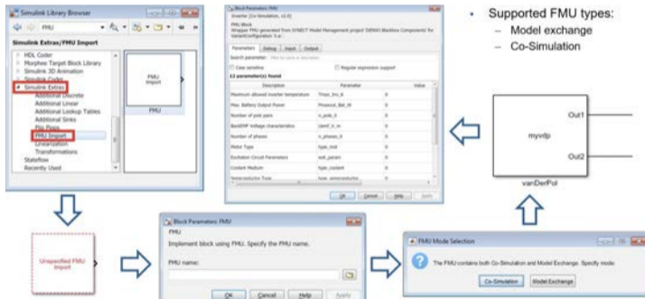
FMU import in Simulink. Source: MathWorks.
