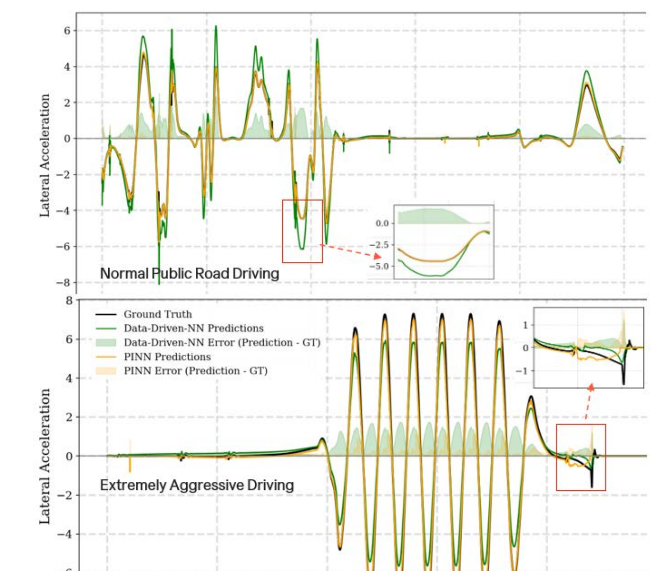
Figure 2. Result on Lateral Acceleration
