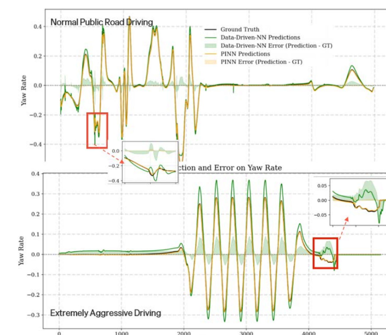
Figure 1. Result on YawRate
