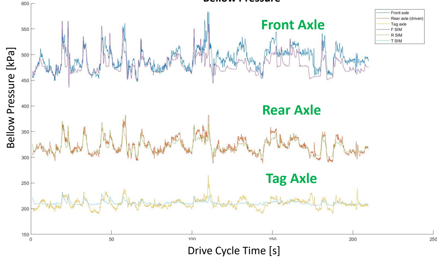
Bellow Pressure
