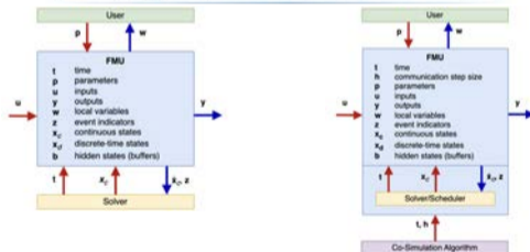
FMI & FMU illustrations. Source: FMI Standard.
