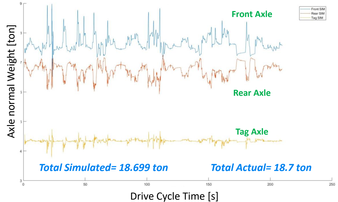
Axle Normal Load
